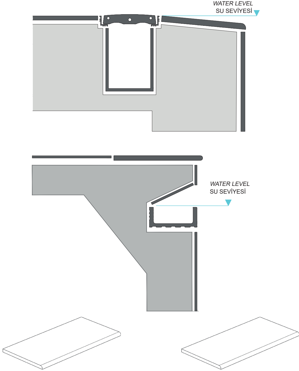
Porcelain Pool Coping Porselen Tutamak
